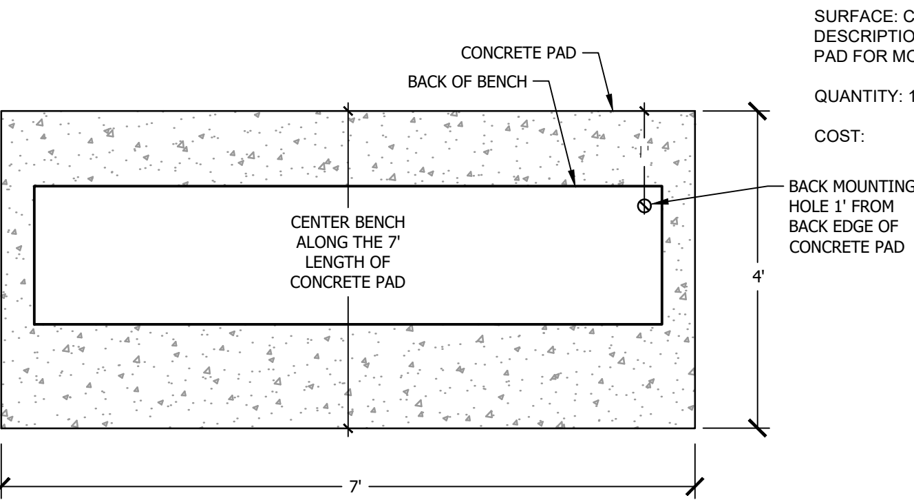
SURFACE - CONCRETE PAD FOR BENCH - PLAN VIEW
